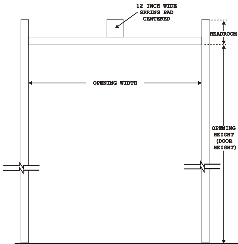
INTERIOR ELEVATION
