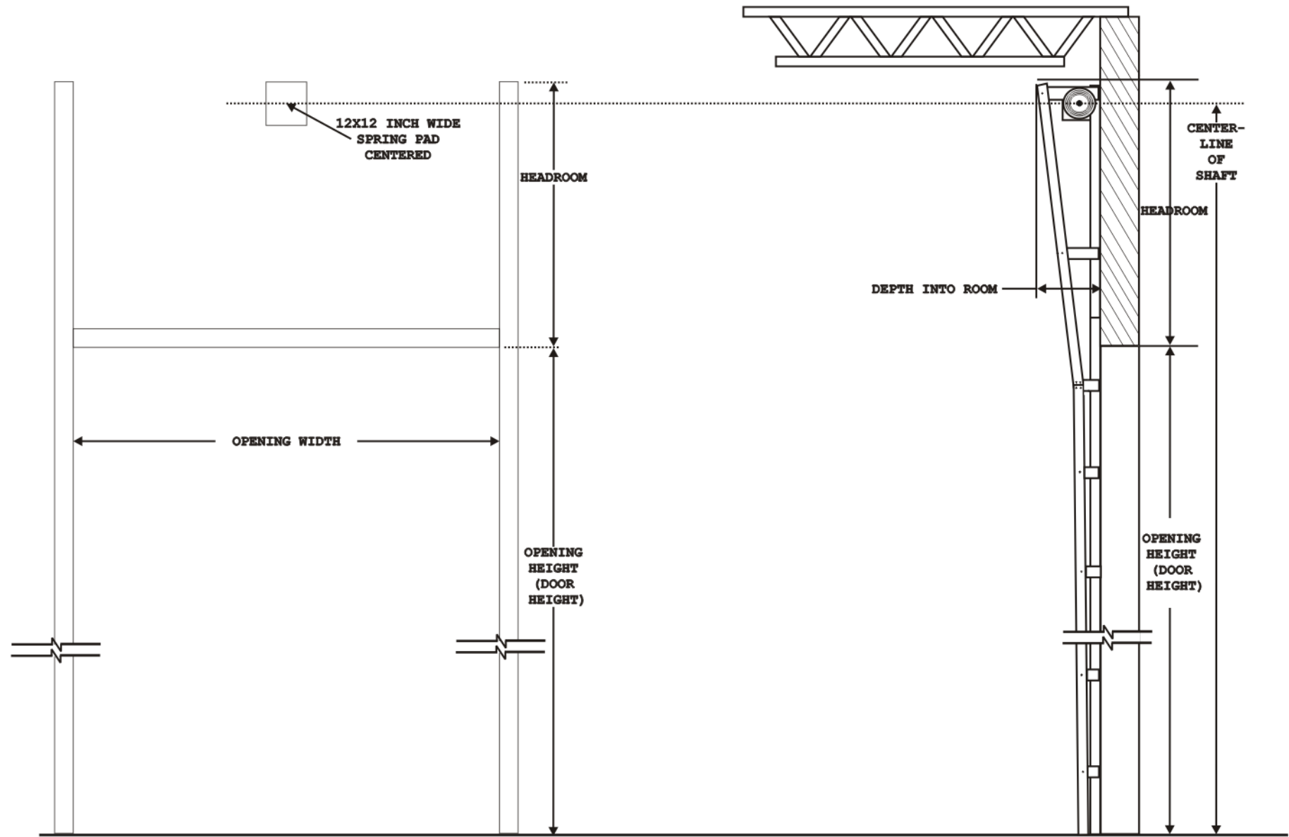
INTERIOR ELEVATION
