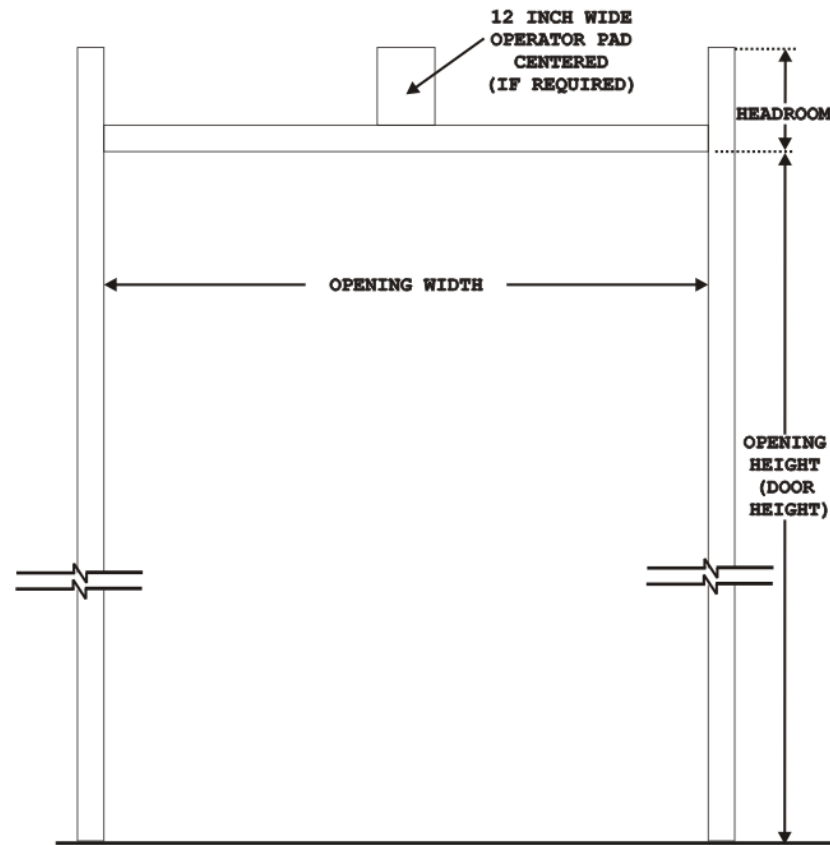
INTERIOR ELEVATION
